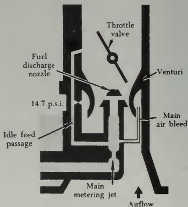
FIGURE 3-8. Main metering system.
